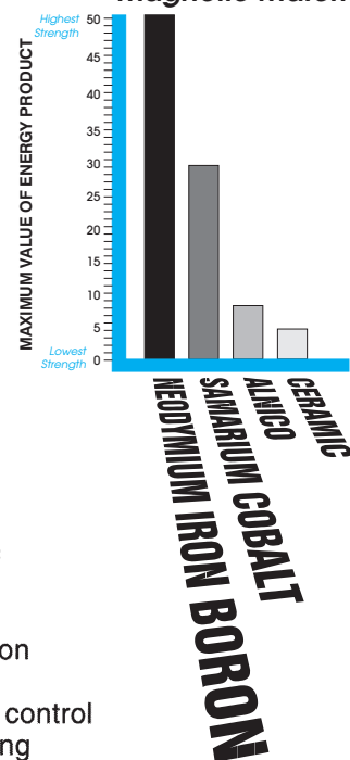
Relative strength of magnetic materials
