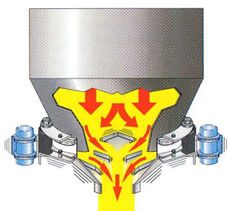
SiloTray Bin Activator Controlled Rate Feeding from a Silo
