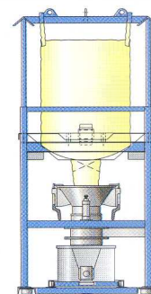
Bulk Bag Unloading System FlexWall has Large Inlet Diameter
