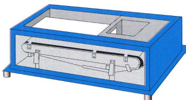
Weigh Belt Feeder 6", 14", 24" and 30" Wide belts
