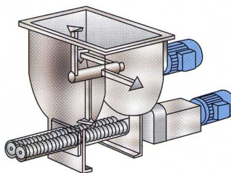
Twin Screw Feeder 12, 20, 40, 60 mm Twin Concave Screws
