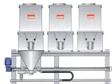
BatchMaster System To 30 Ingredients, Travelling Scale Hopper
