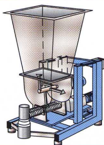
Loss-in-Weight Agitated Screw Feeder Internal Agitation for some Ingredients
