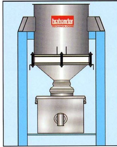
Volumetric feeding using a FlexWall™ discharge feeder.
