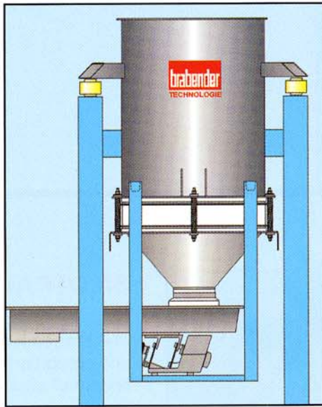
Gravimetric feeding using a vibrating tray discharge feeder.
