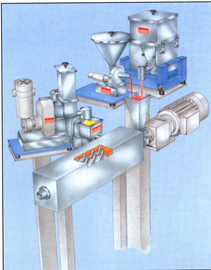
Lab Size Extrusion Line with Brabender Micro Feeders
