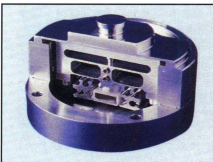
Fast Deflectionless Weighing: IDL-F and Frame Scale combine for immediate response, 8/1000 inch movement from full to no load.
